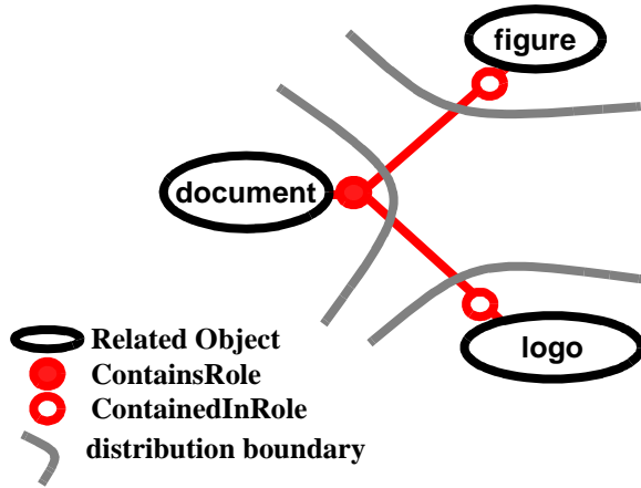
FIGURE 6. Clustering roles with the related objects
