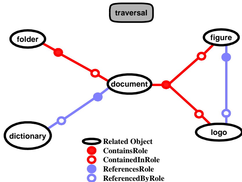
FIGURE 8. An example graph of related objects. The folder contains the document; the document references the dictionary and contains the figure and the logo; the figure references the logo.
