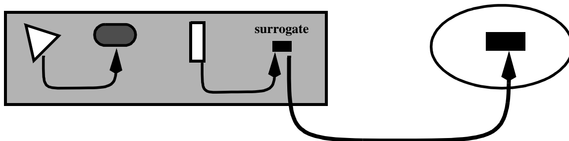
FIGURE 1. A distributed object system allows objects to request the services of other objects, possibly across heterogeneous system boundaries. On the left, an object requests the services of another object in the same system. On the right, an object requests the service of an object in another system by way of a surrogate object.
