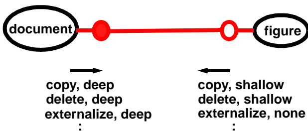
FIGURE 10. Propagation attributes for the containment relationship
